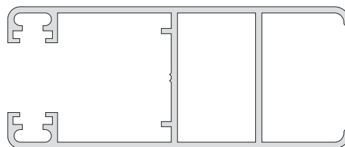
3050 / 425 Parante 707 grs/mt. 8 barras 6.150
